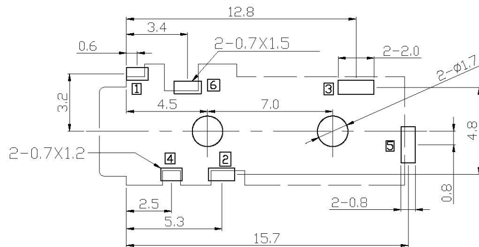
P.C.B LAYOUT BOTTOM VIEW
