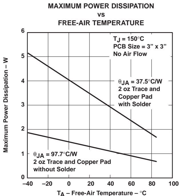
Figure 59. Maximum Power Dissipation vs Free-Air Temperature
