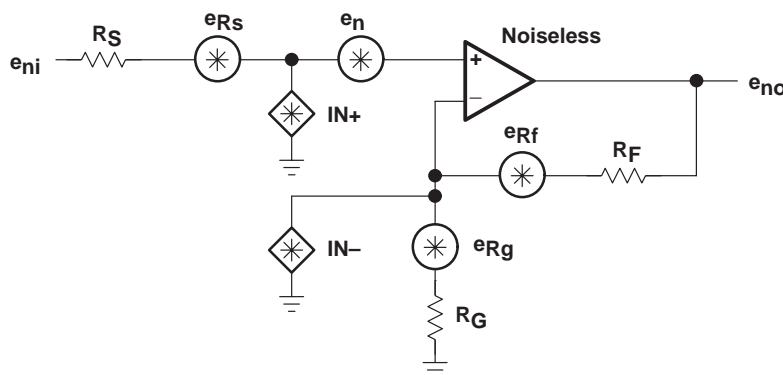
Figure 51. Noise Model
