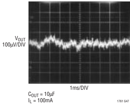
LT1761-5 10Hz to 100kHz Output Noise C_{BYP} = 1000\text{pF}
