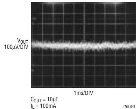
LT1761-5 10Hz to 100kHz Output Noise C_{BYP} = 0.01\mu\text{F}
