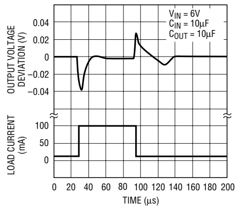
LT1761-5 Transient Response C_{BYP} = 0.01\mu\text{F}
