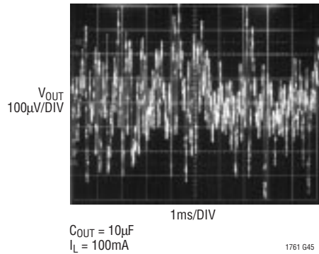
LT1761-5 10Hz to 100kHz Output Noise C_{BYP} = 0
