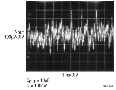
LT1761-5 10Hz to 100kHz Output Noise C_{BYP} = 100\text{pF}
