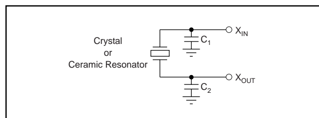
FIGURE 2. Crystal or Ceramic Resonator Connection.
