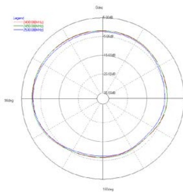
ZY plane
