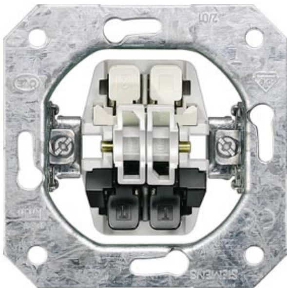
DELTA SWITCH INSERT FM SHUTTER SWITCH 16A 250V MECHANICALLY INTERLOCKED
