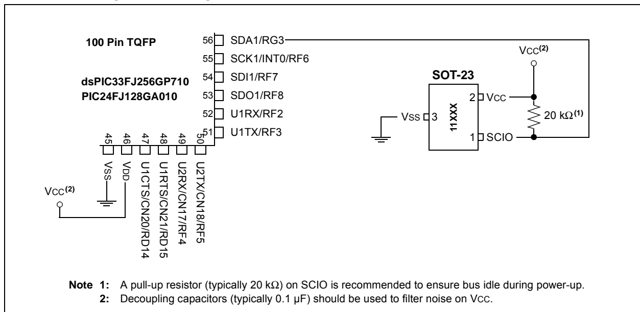
FIGURE 1: CIRCUIT FOR dsPIC33FJ256GP710 OR PIC24FJ128GA010 AND 11XXX SERIAL EEPROM
