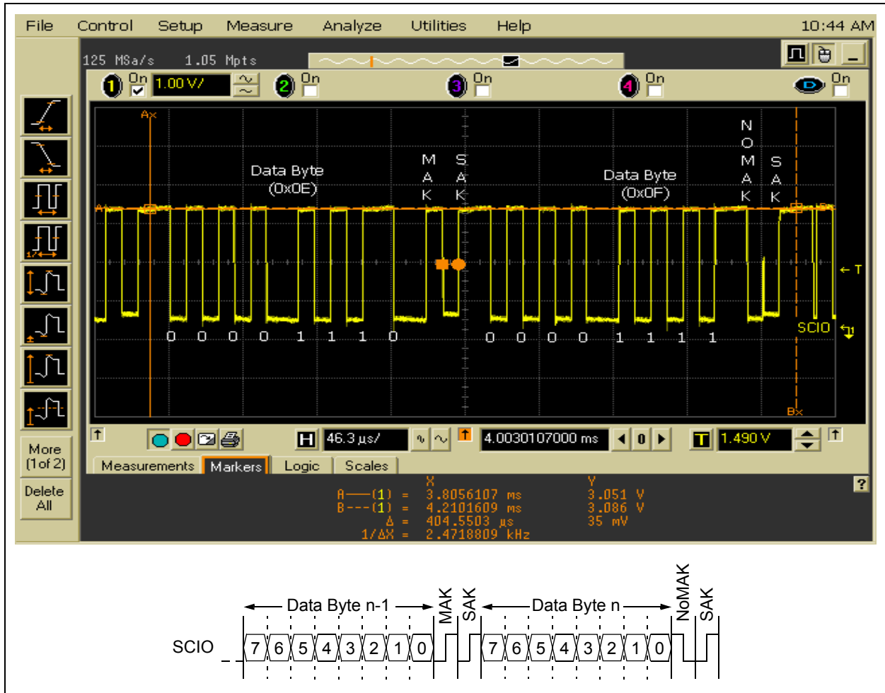
FIGURE 6: WRITE COMMAND FINAL TWO DATA BYTES
