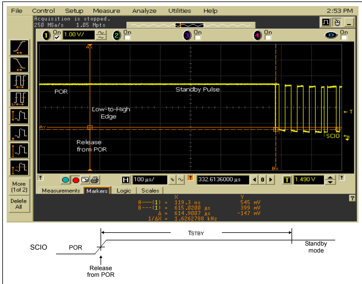
FIGURE 2: STANDBY PULSE
