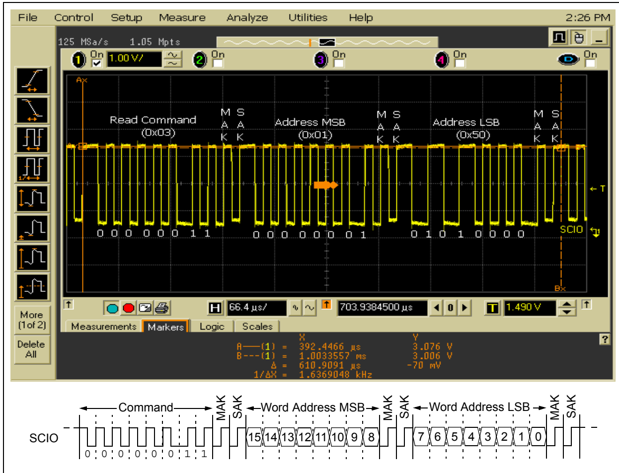
FIGURE 9: READ – COMMAND BYTE AND WORD ADDRESS
