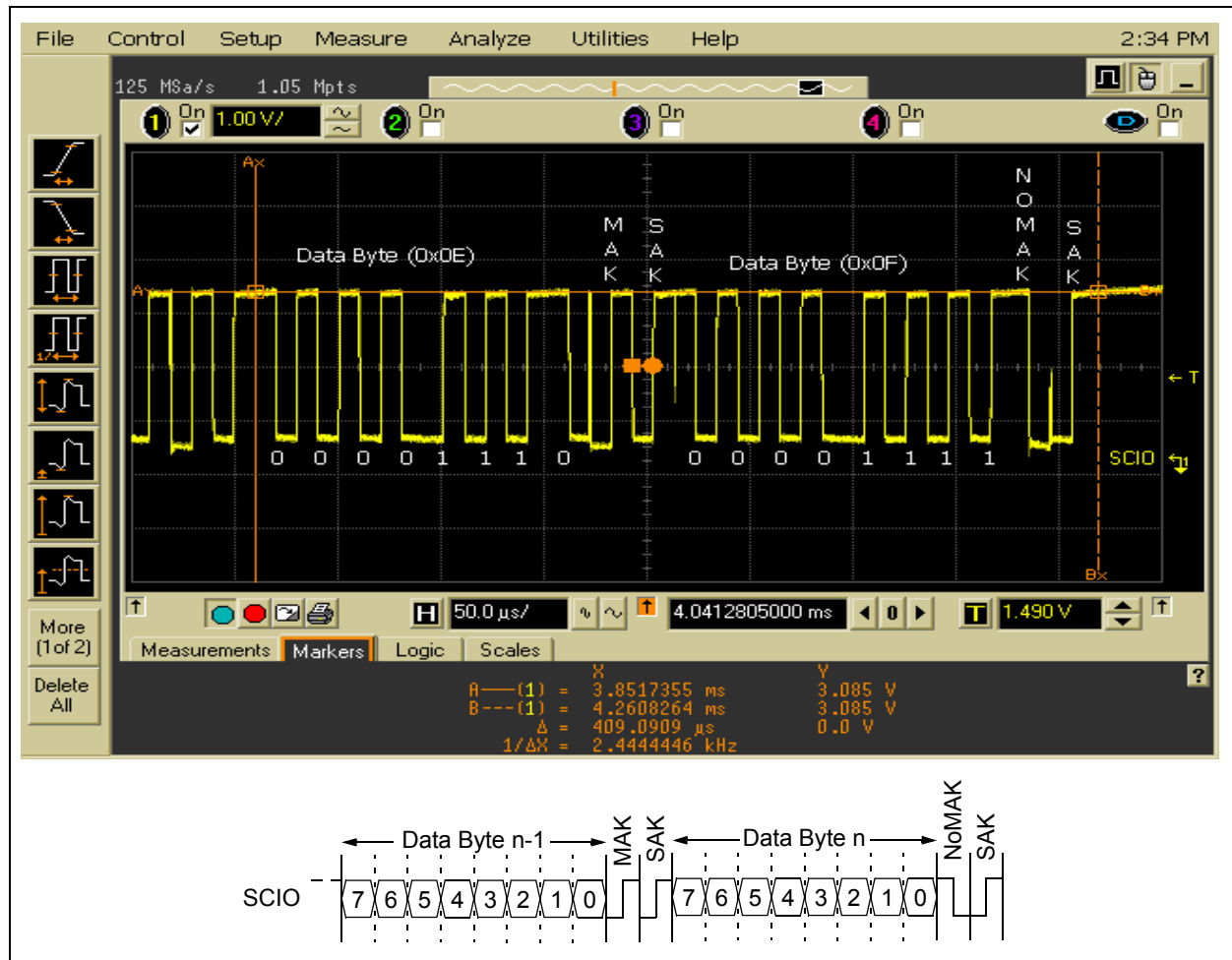
FIGURE 10: READ – FINAL TWO DATA BYTES
