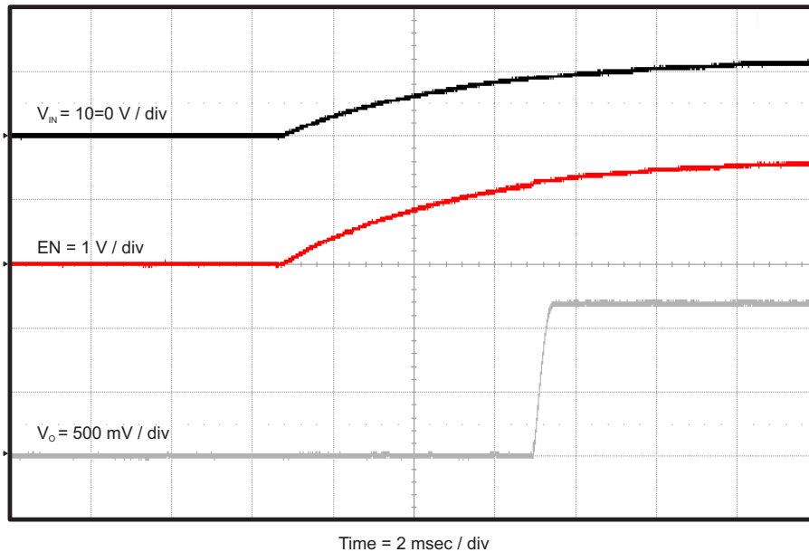
Figure 13. TPS54A20EVM-770 Start-Up Relative to V_{IN}
