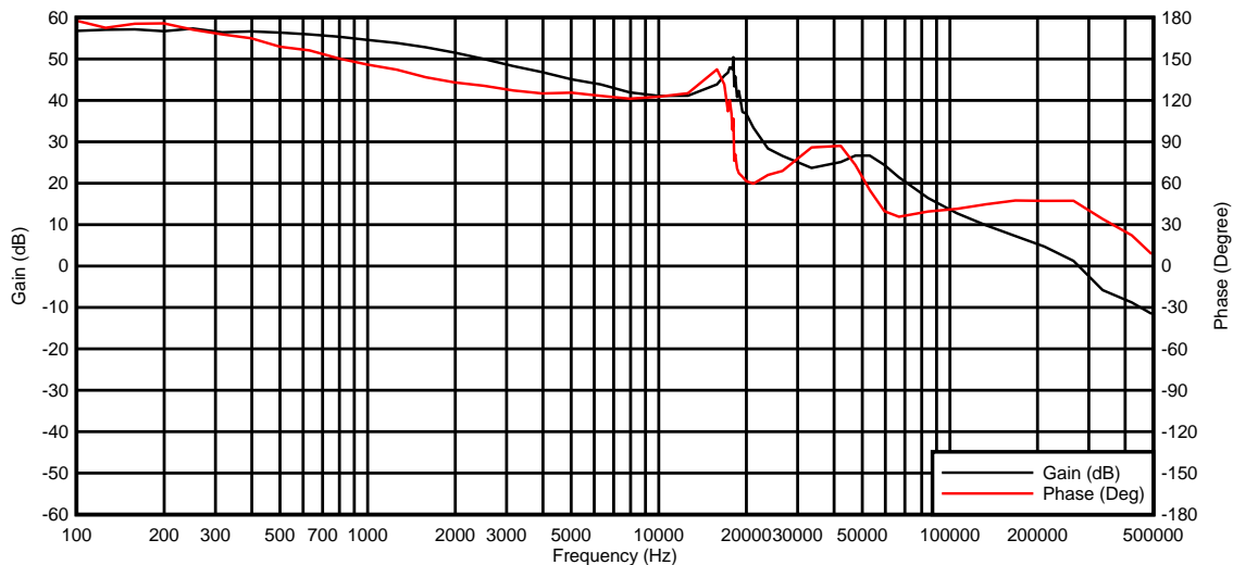
Figure 6. TPS54A20EVM-770 Loop Response
