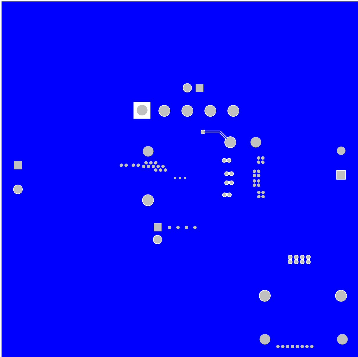
Figure 20. TPS54A20EVM-770 Bottom-Side Layout
