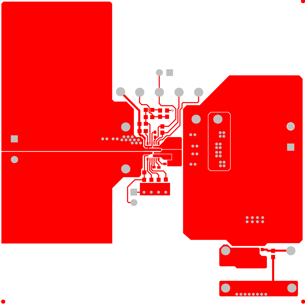
Figure 17. TPS54A20EVM-770 Top-Side Layout
