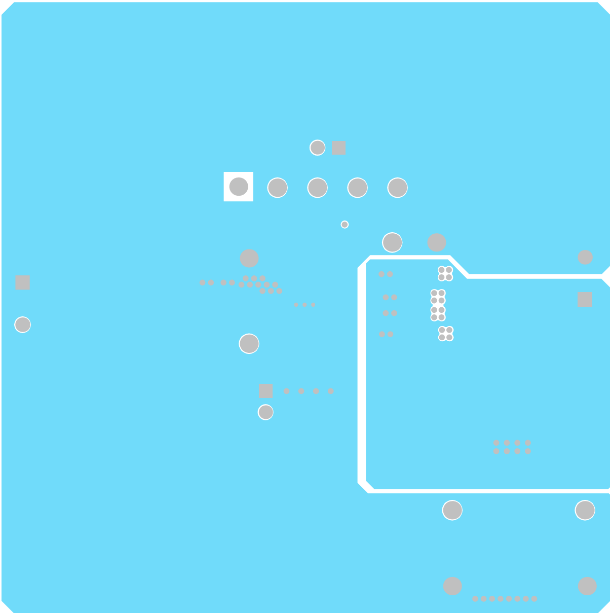
Figure 19. TPS54A20EVM-770 Internal Layer-2 Layout
