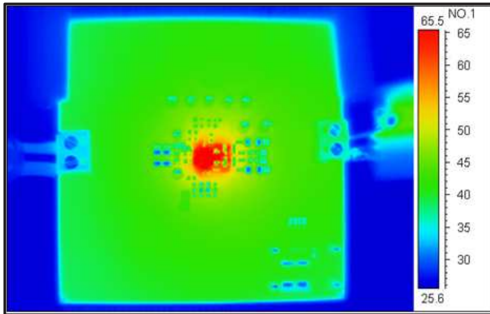
Figure 15. Thermal Image
