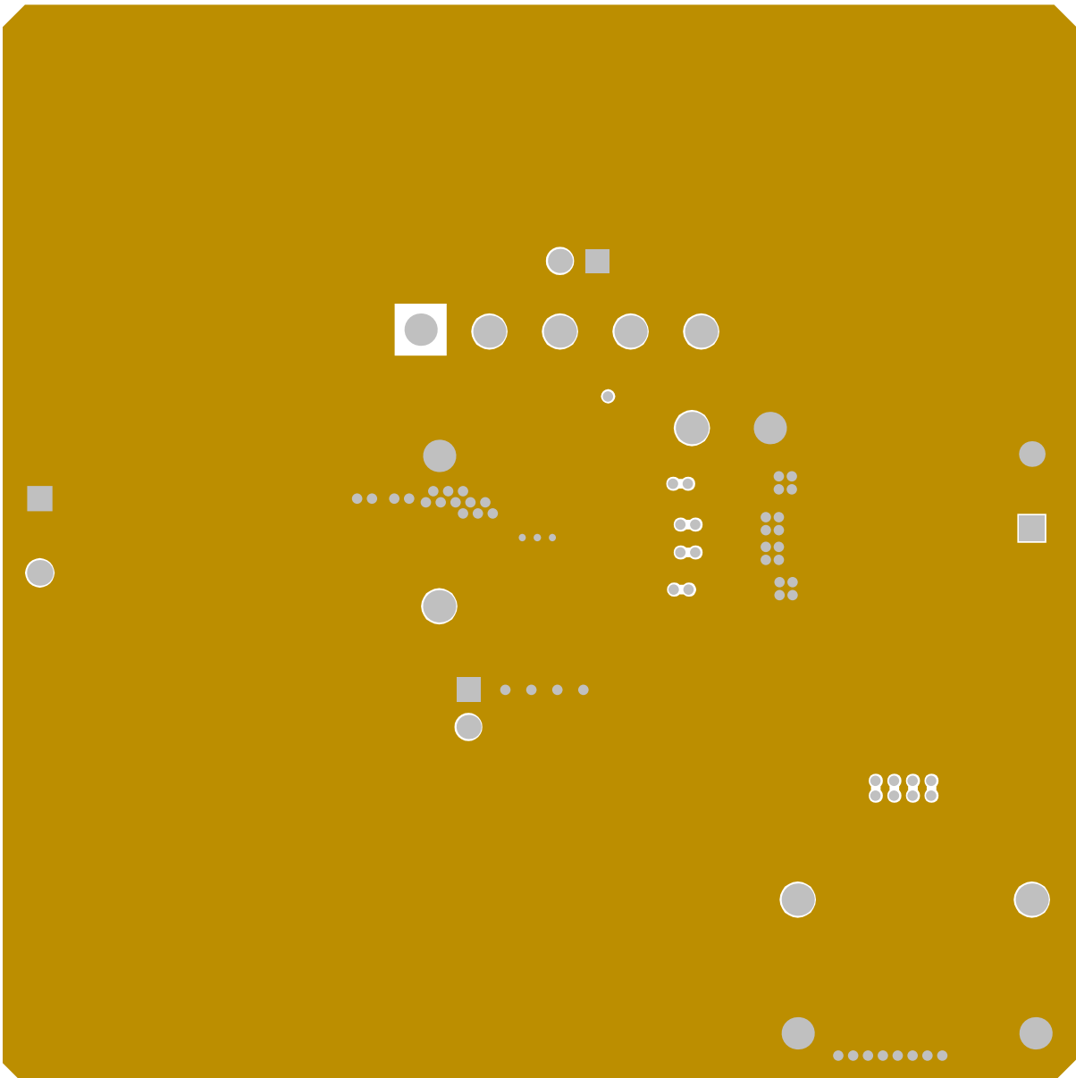
Figure 18. TPS54A20EVM-770 Internal Layer-1 Layout
