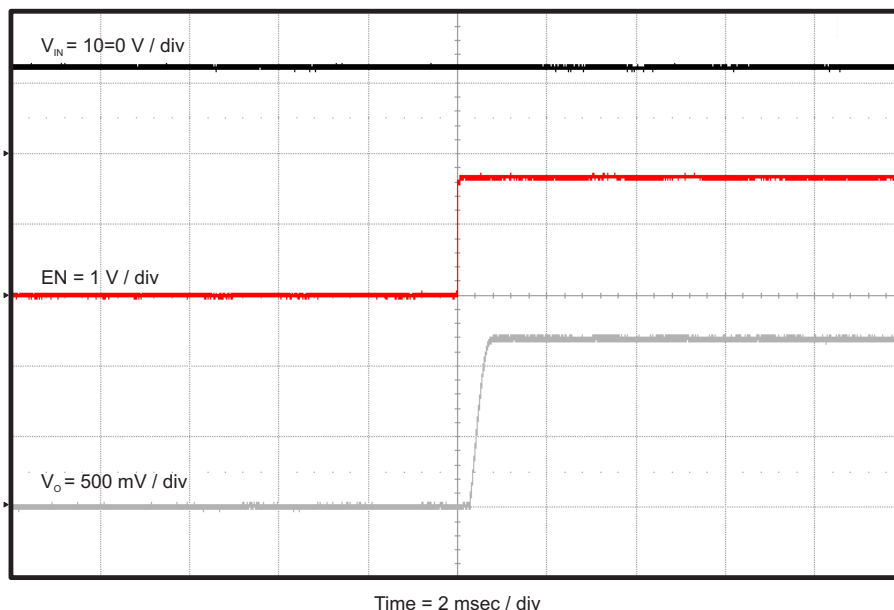
Figure 14. TPS54A20EVM-770 Start-Up Relative to Enable
