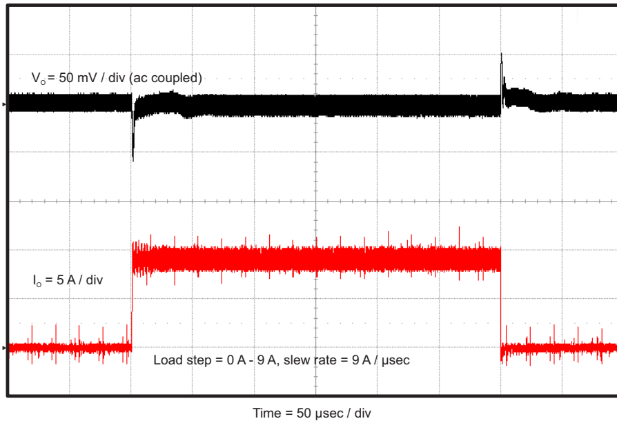
Figure 5. TPS54A20EVM-770 Transient Response
