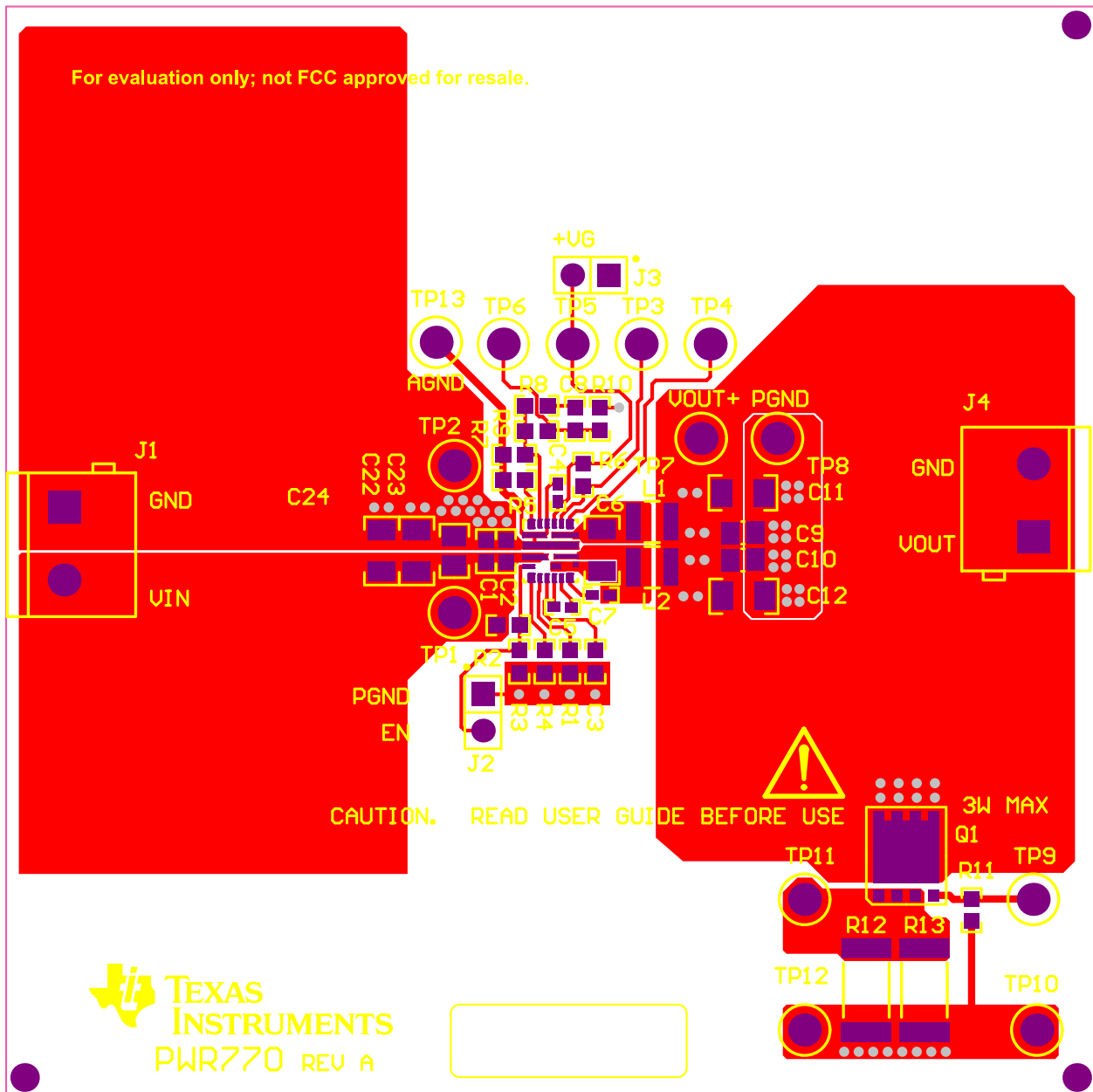
Figure 16. TPS54A20EVM-770 Top-Side Assembly
