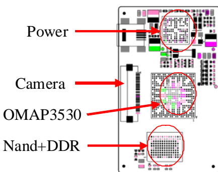
Embest Mini8100 Layout
